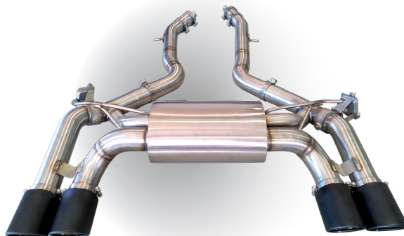
BM.002.C01 REAR EXHAUST WITH VALVES COMPLETE WITH BLACK CHROME TEALPIPE 90 MM
