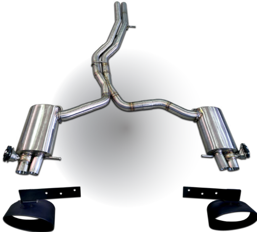
AU.005.C01 COMPLETE EXHAUST SYSTEM FROM CENTRAL TO REAR WITH VALVES + MATT BLACK OVAL TAILPIPES
