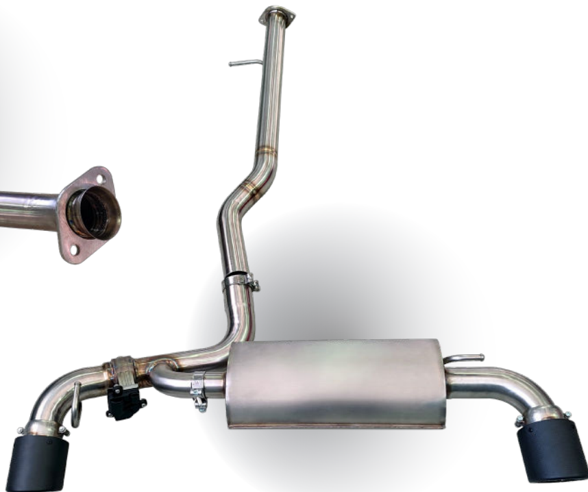
TO.003.C01 REAR EXHAUST WITH ELECTRIC VALVES COMPLETE WITH BLACK CHROME TEALPIPE DIAMETER 100 mm
